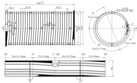
Crossover Grooved drum sleeves for PWK12600
