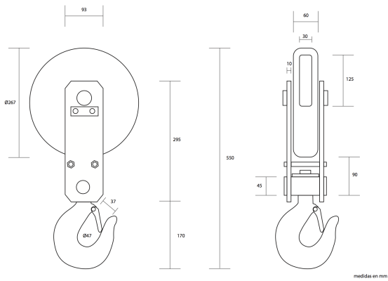
Hook block with pulley for PWMD3T24M
